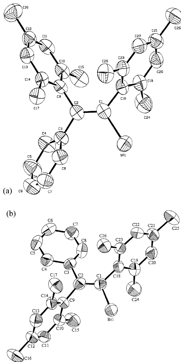
Figure 3. ORTEP drawings of (a) E-4-Br , and (b) one form of Z-4-Br
