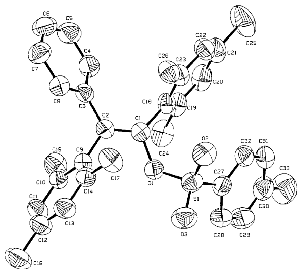
Figure 1. ORTEP drawing of Z-4-OTs
