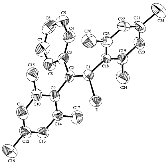
Figure 2. ORTEP drawing of one form of Z-4-I
